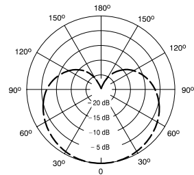
1000 Hz
