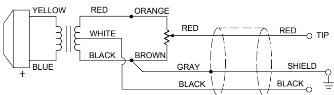
INTERNAL CONNECTIONS UNBALANCED HIGH-IMPEDANCE OUTPUT FIGURE 3
