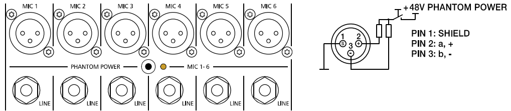
Illustration 2-1: Microphon input
