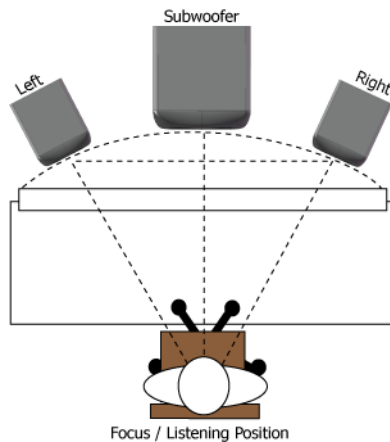
Figure 4.0 – Subwoofer Placement
