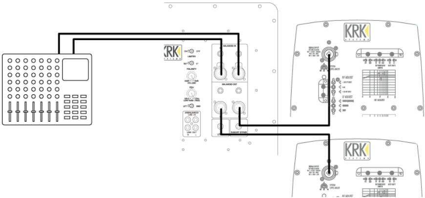
Figure 3.1 – Subwoofer Hookup with Active Studio Monitors
