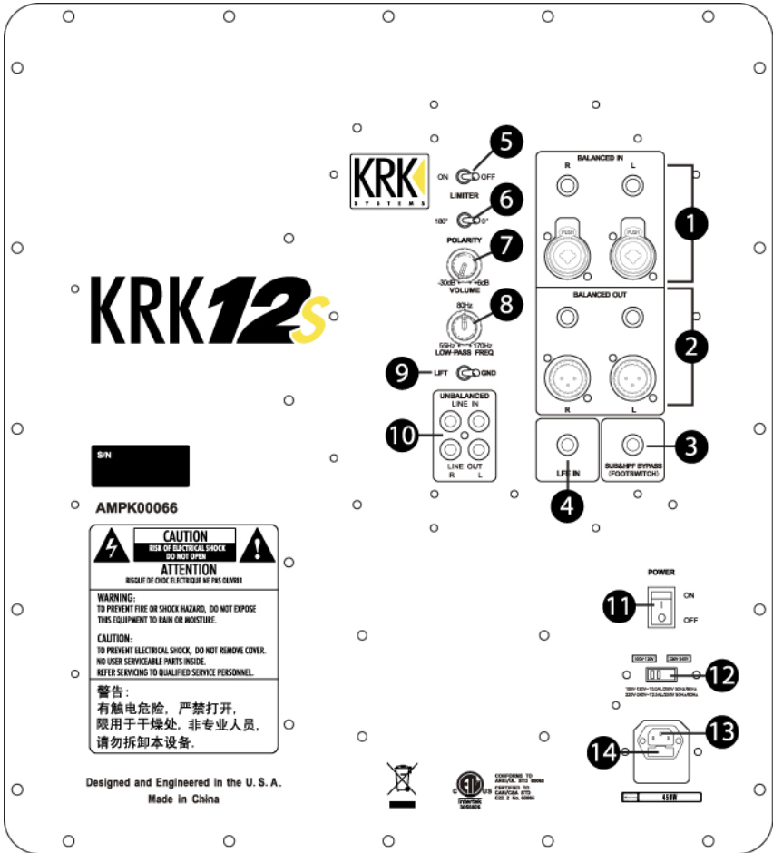
Figure 2.1 – System Controls on the Rear Panel
