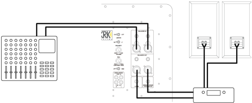
Figure 3.2 – Subwoofer Hookup with Passive Studio Monitors
